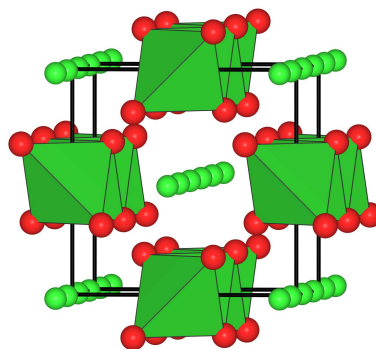
TlSe (Polyeder-Darst.)
