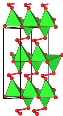
In 2 Te 5
