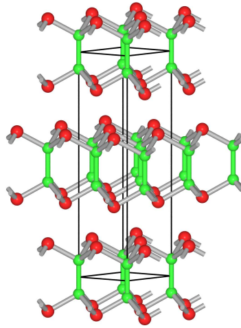
GaSe
