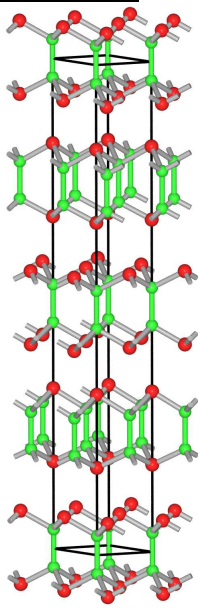
GaSe
