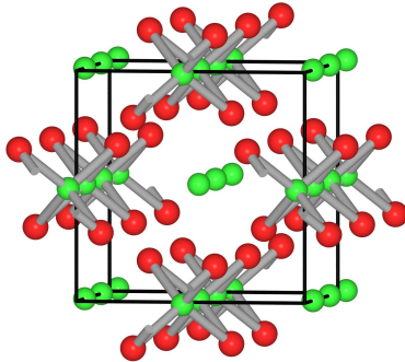
TlSe (Stick-and-Ball-Darst.)
